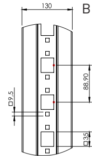
Detail B
