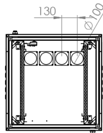
Top/inside view
