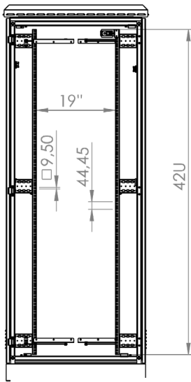
Front/inside view
