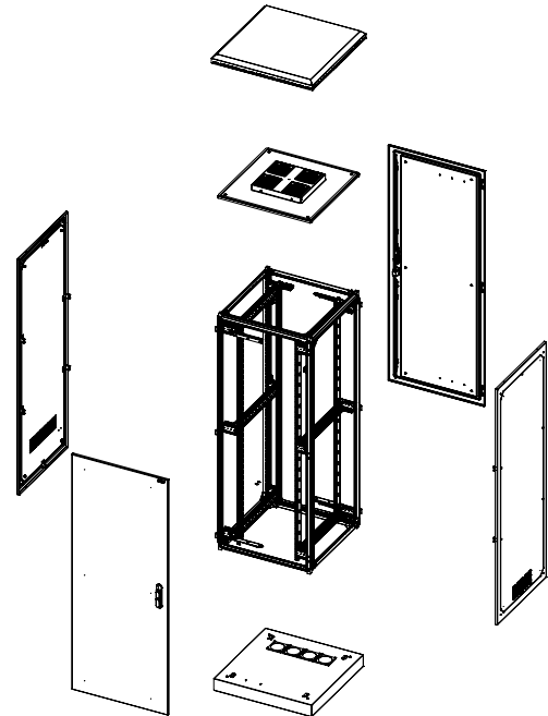
Exploded view
