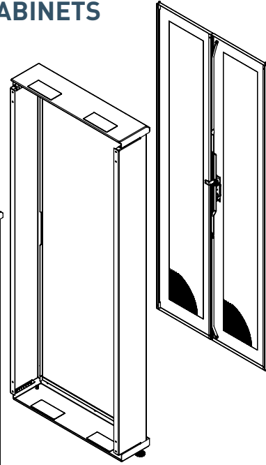
Exploded view
